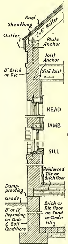
Wall Section
